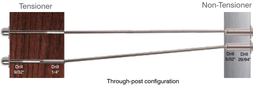
Through-post configuration
