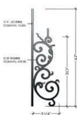
TOP VIEW B-2 ALL RADIUS FROM 30\"/> HFBX.B2
