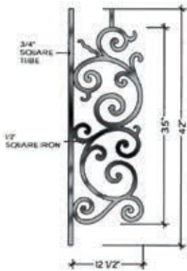
TOP VIEW A-2 ALL RADII FROM 28" TO 20'-0" HFM0.A2
