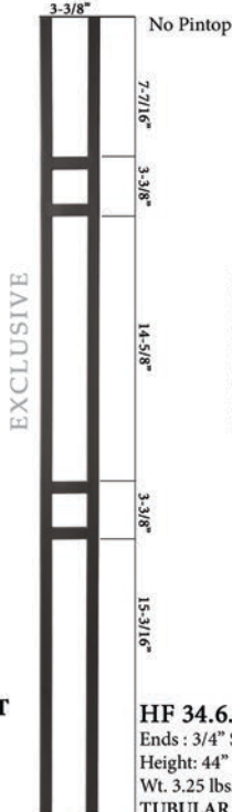
HF 34.1.35-T Ends : 3/4" Sq. Height: 44" Wt. 2 lbs. TUBULAR
