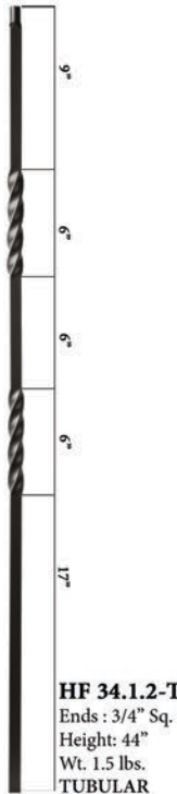
HF 34.1.1-T Ends : 3/4" Sq. Height: 44" Wt. 1.5 lbs. TUBULAR
