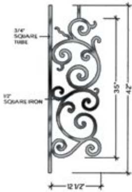
TOP VIEW A-2 ALL RADII FROM 28" TO 20'-0" HFMO.A2
