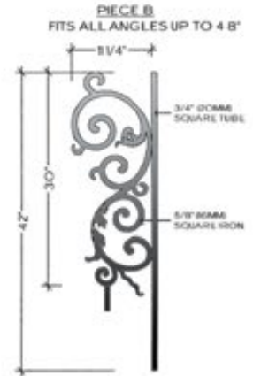
TOP VIEW B-1 FLAT HFBX.B1
