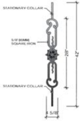
PIECE F FITS LEVEL BALCONY OR STRAIGHT RAIL
