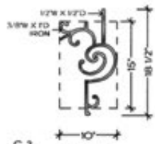
C-2 TOP VIEW FLAT
